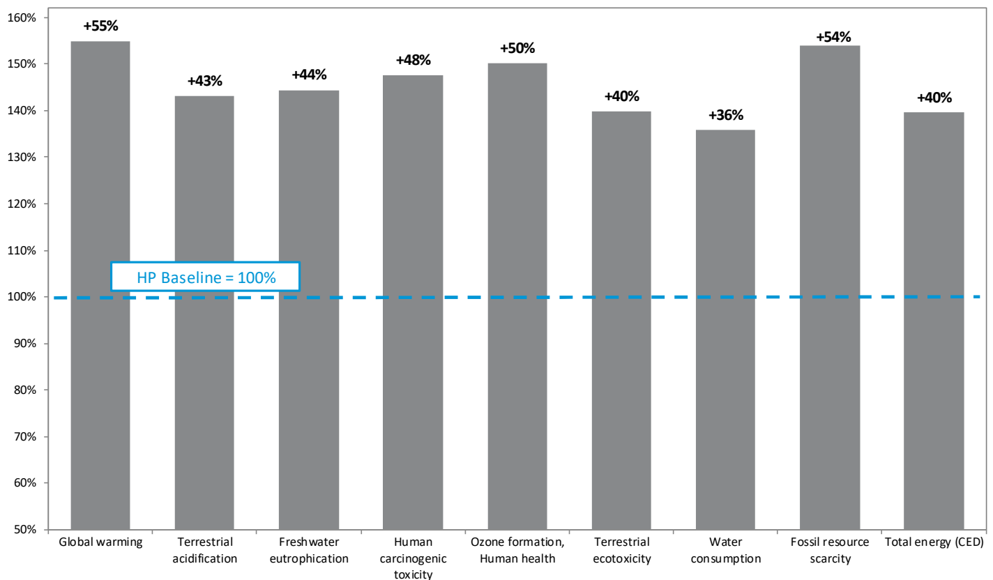
Figure 2 NBC Results Compared to HP Results
