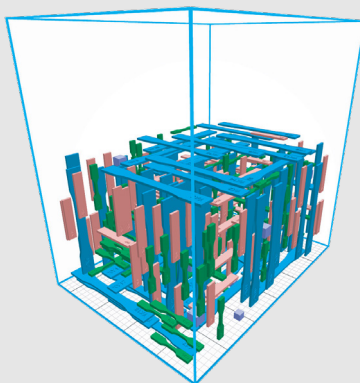
Figure 1. “Half_Commercial_Datasheet_Job” part property test job
