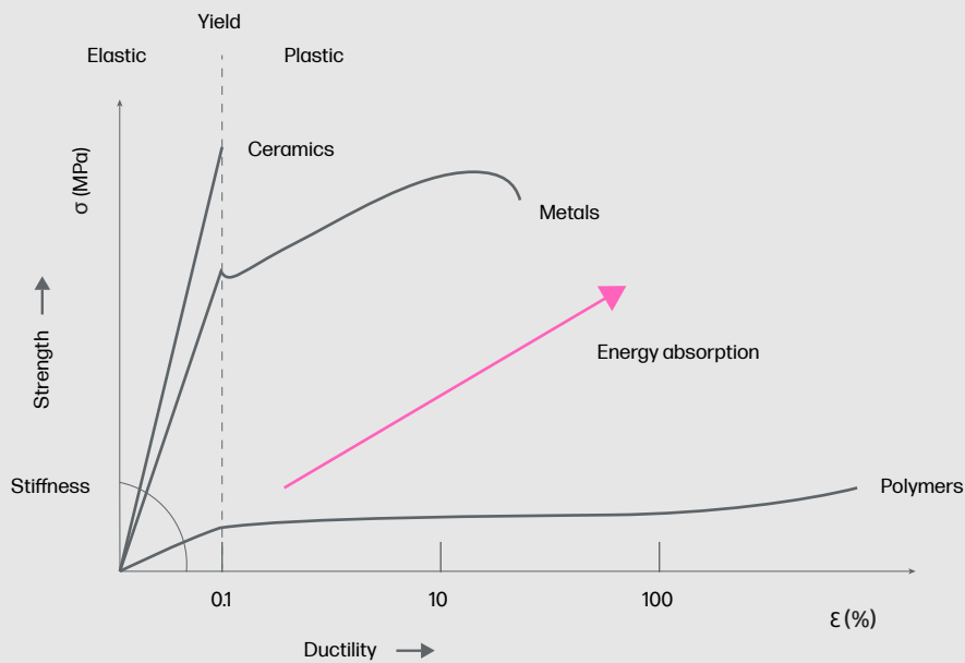
Figure 3. Comparison of polymer, metal, and ceramic materials
